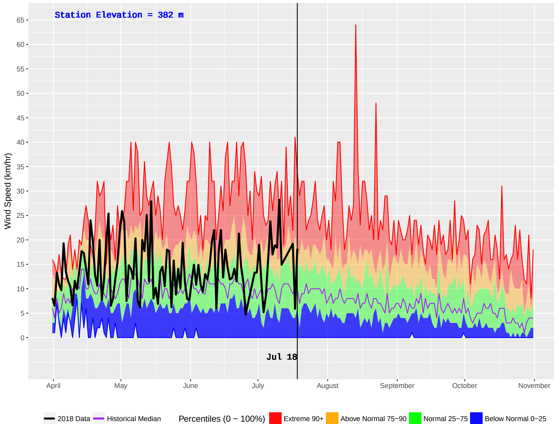
TELEGRAPH CREEK (110) : Historical (1978–2016) and Current (2018) Daily Wind Speed
